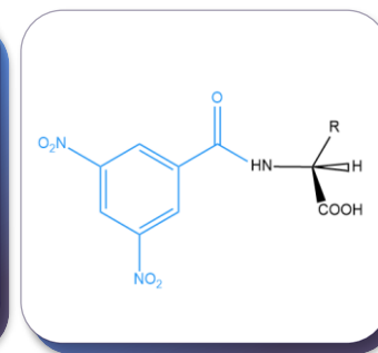
N-3,5-dinitrobenzoyl
