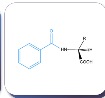
N-benzoyl
